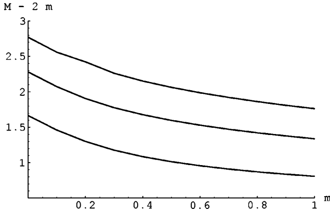
FIG. 1. Dependence of the differences M - 2m of the eigenvalues M of the instantaneous Bethe-Salpeter equation and the sum of the masses m of the bound-state constituents for the three lowest-lying J^{PC} = 0^{-+} bound states, obtained from a time-component Lorentz-vector confining interaction kernel involving a linear potential V(r) = \lambda r with slope \lambda = 0.2 \text{ GeV}^2 , on the bound-state constituents' mass m (all masses in units of GeV). The chosen truncation parameters are N = 49 in the intermediate series expansions as well as d = 15 for the matrix size (except for m = 0.1 \text{ GeV} , where, in order to increase the accuracy, d = 50 has been used).
